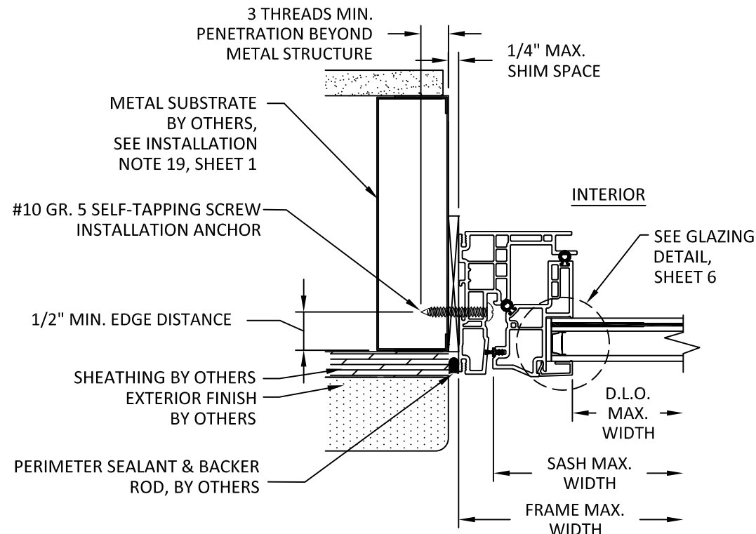
B-4 HORIZONTAL SECTION THROUGH FRAME INSTALLATION METAL SUBSTRATE
