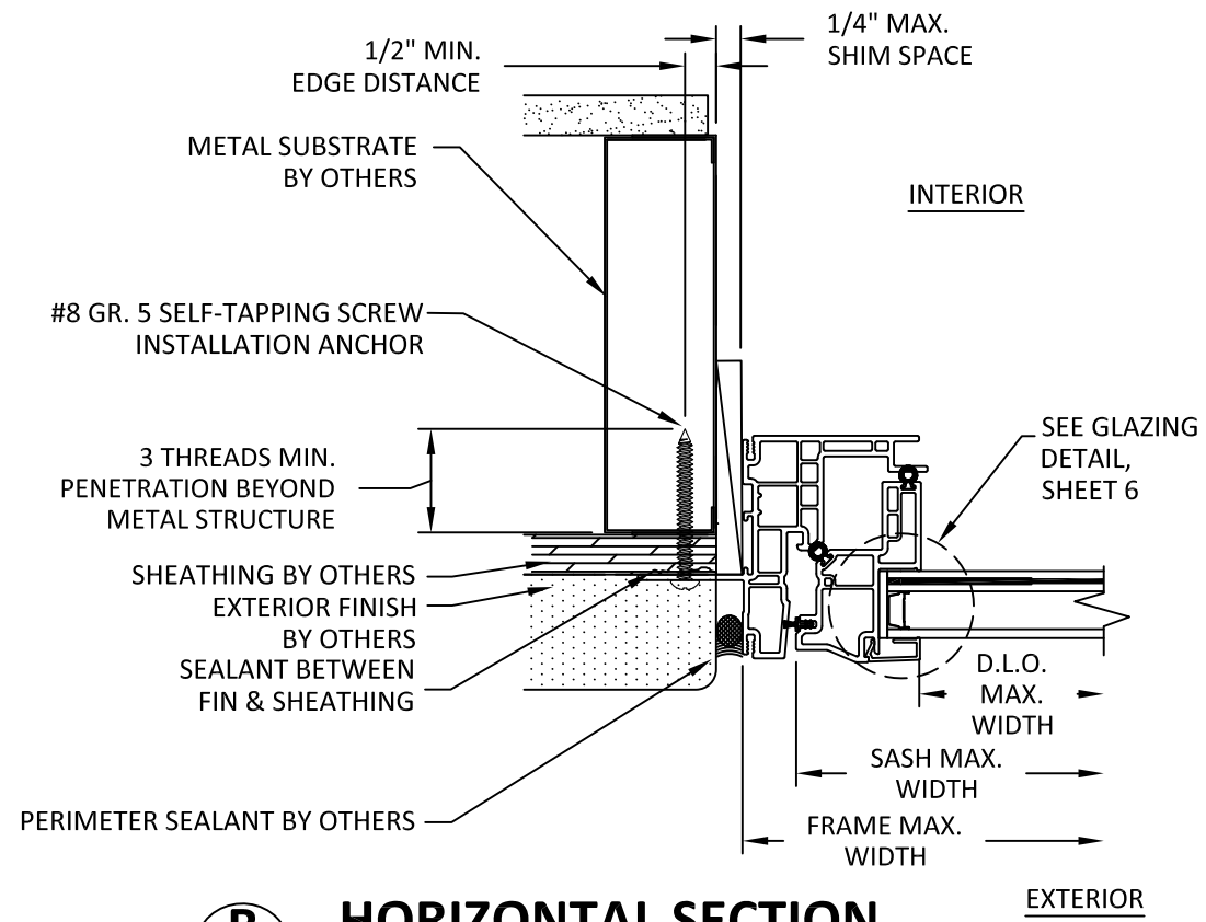
B 3 HORIZONTAL SECTION NAIL FIN INSTALLATION METAL SUBSTRATE
