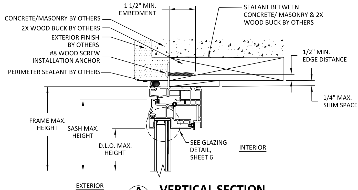
A 3 VERTICAL SECTION NAIL FIN INSTALLATION WOOD SUBSTRATE
